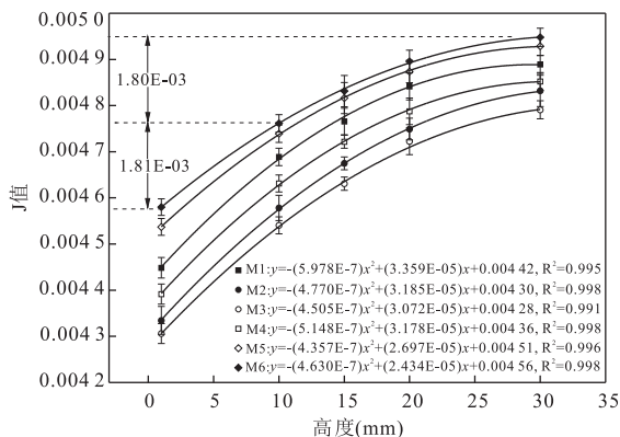
图 4 不同径向位置的轴向方向中子通量梯度变化曲线 Fig.4 Curves about the neutron flux gradient along with the axial direction at different radial positions
