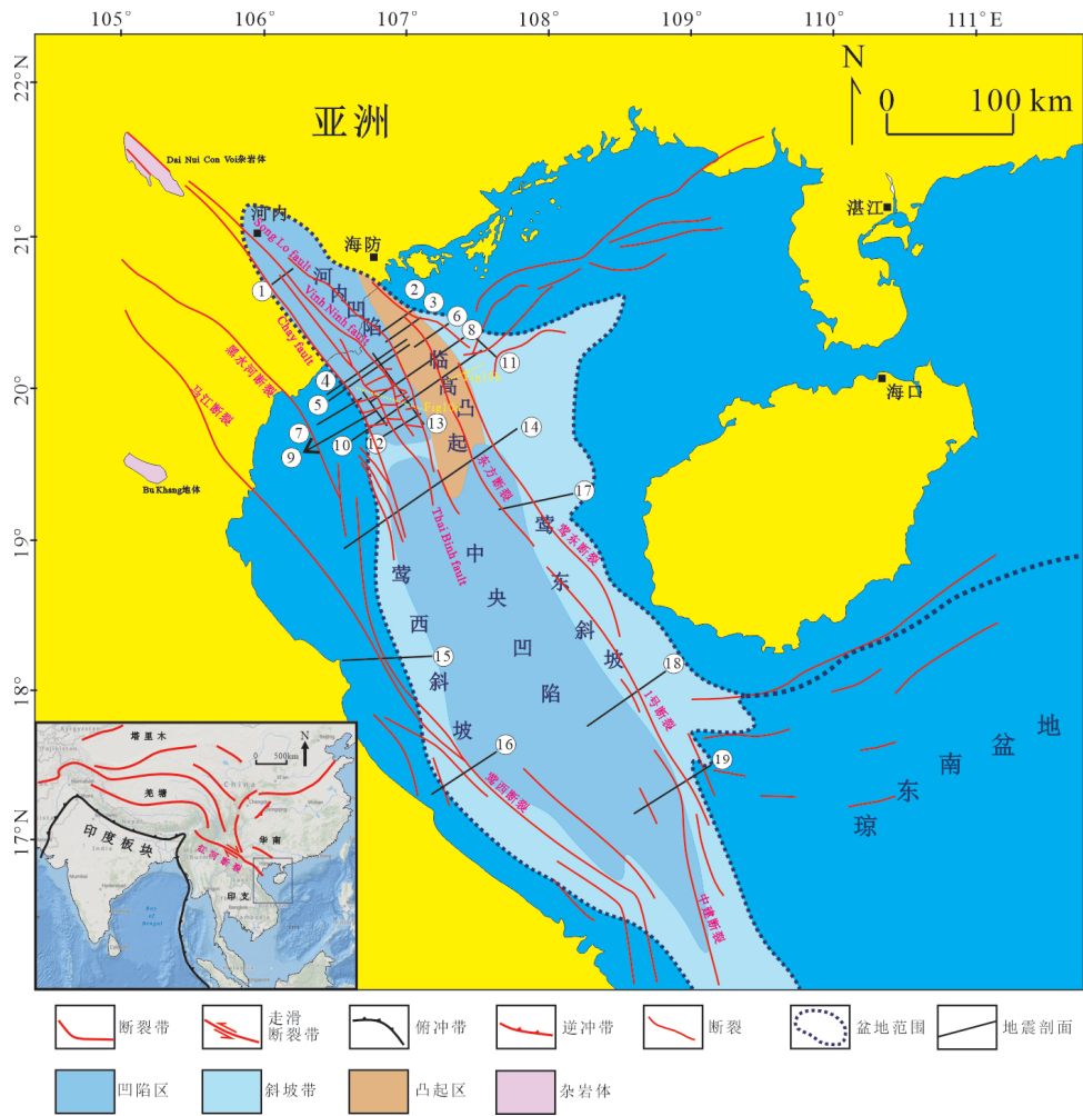
图1 莺歌海盆地的构造格架 Fig.1 Tectonic framework of the Yinggehai Basin
