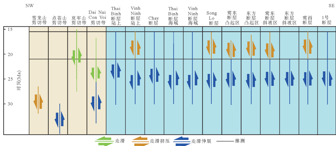
图9 哀牢山—红河剪切带及莺歌海盆地断层运动特征(雪龙山、点苍山、哀牢山和 Dai Nui Con Voi, 资料据 Morley et al. , 2023) Fig.9 Fault movement characteristics of the Ailaoshan-Red River Shear Zone and Yinggehai Basin(data is based on Morley et al. , 2023)
