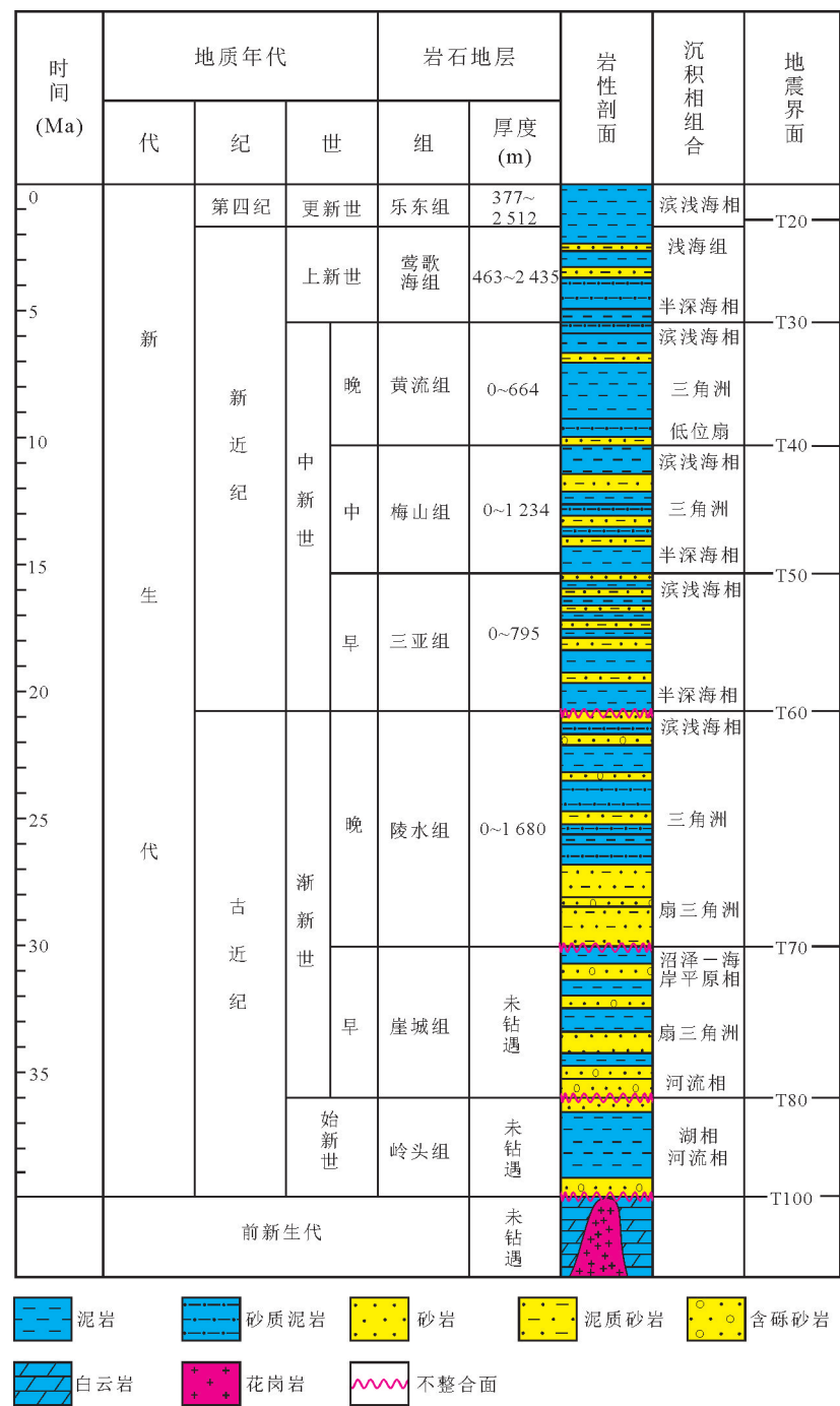
图3 莺歌海盆地综合柱状图(据解习农等, 2009修改) Fig.3 Stratigraphic division of the Yinggehai Basin(modified from Xie et al. , 2009)
