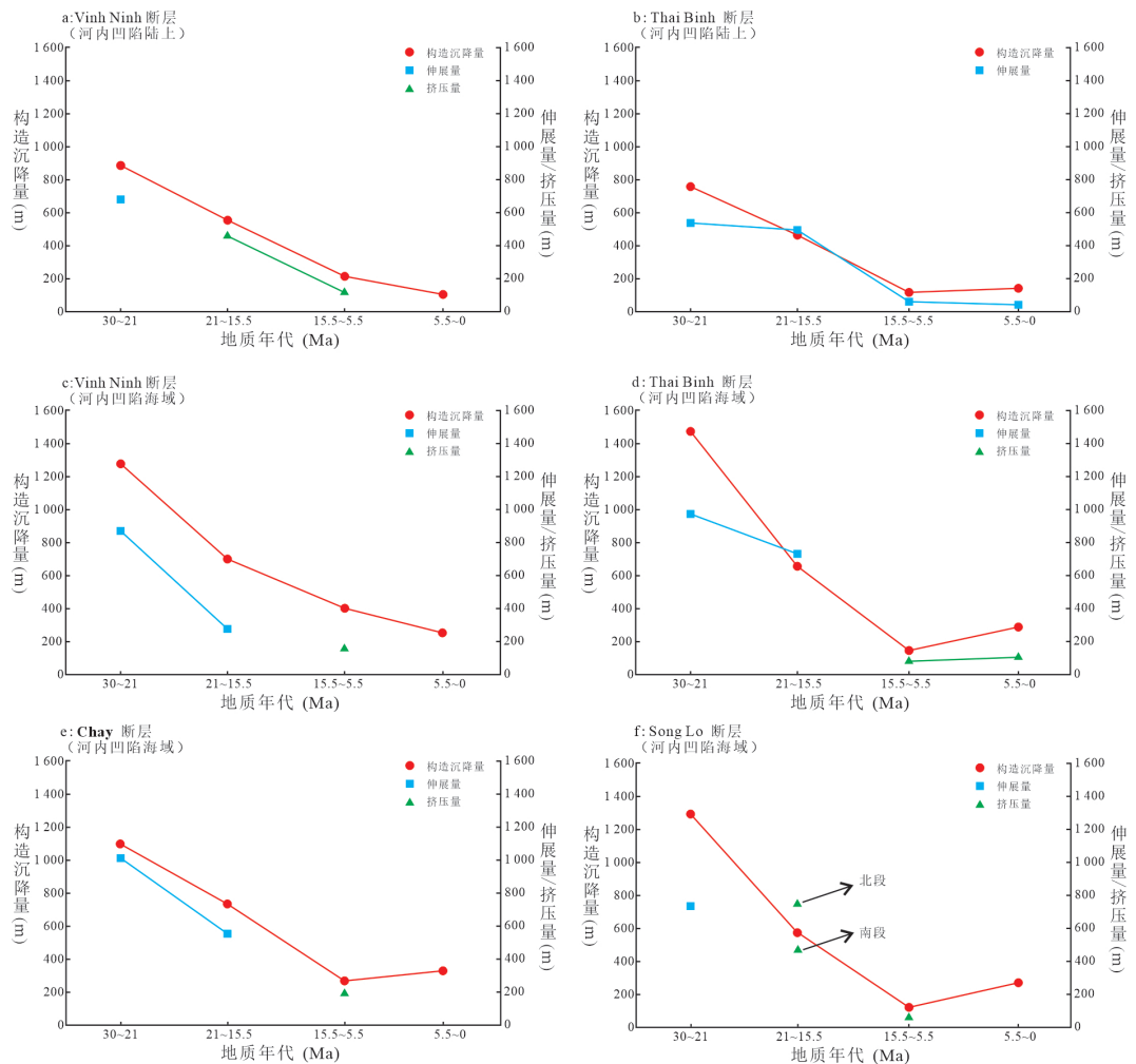
图4 莺歌海盆地河内凹陷主要断层活动性 Fig.4 The tectonic subsidence and extension (compression) amounts of faults in the Ha Noi Depression
