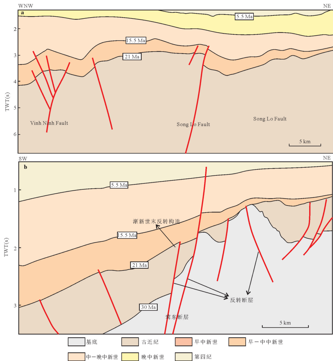
图 11 构造反转类型(剖面位置见图 1) Fig.11 Types of inversion in the Yinggehai Basin(See section location in Fig.1)
