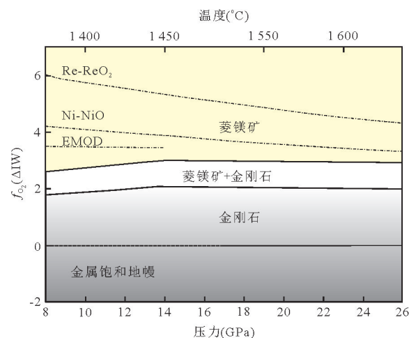
图1 地幔内部碳的赋存形式随地温梯度、压力和氧逸度的演化 Fig.1 Evolution of carbon speciation in the Earth's mantle as a function of geothermal gradient, pressure, and oxygen fugacity
