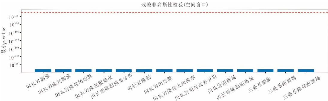
图 6 Shapiro-Wilk (SW) 检验 Fig.6 Shapiro-Wilk (SW) test
