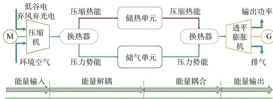
图6 压缩空气储能系统示意(袁照威和杨易凡,2024)
