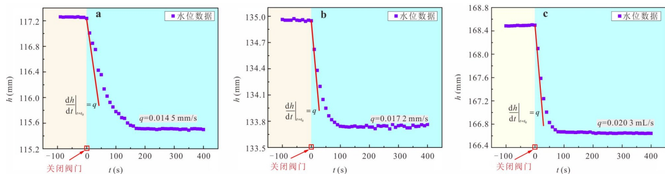
图 5 不同流量下井管内水位—时间动态曲线(地表水补给地下水) Fig.5 The water level-time dynamic curves in the well under different flow rates (surface water recharges groundwater)
