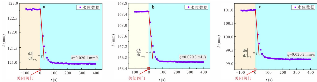
图 7 不同深度下井管内水位—时间动态曲线 Fig.7 The water level-time dynamic curves in the well under different depths
