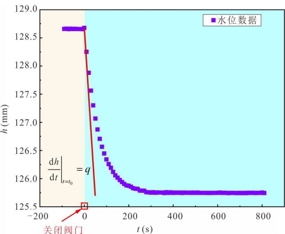
图3 井管内水位—时间动态曲线 Fig.3 Water level-time dynamic curve in the well
