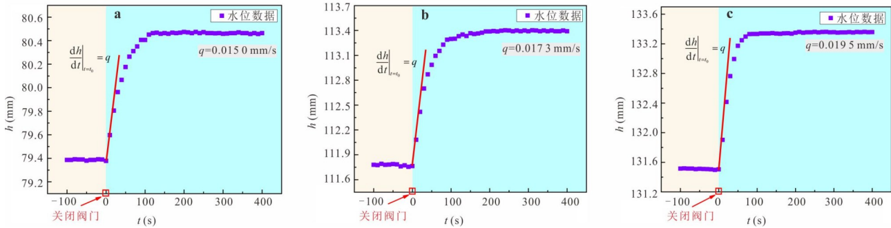
图 6 不同流量下井管内水位—时间动态曲线(地下水补给地表水) Fig.6 The water level-time dynamic curves in the well under different flow rates (groundwater recharges surface water)
