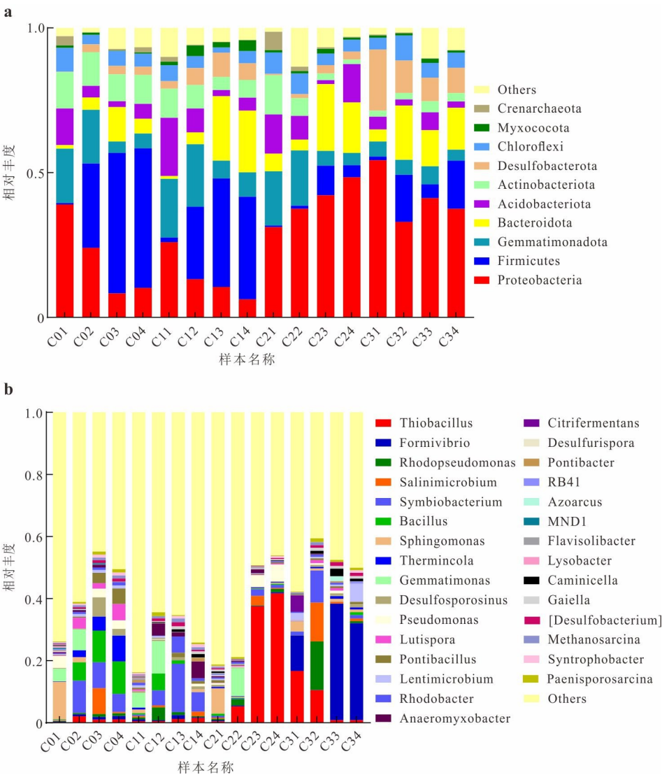
图7 潜流带沉积物样品在门水平与属水平的微生物种群结构 Fig.7 Microbial community members at the phylum level and the genus level in river sediment samples
