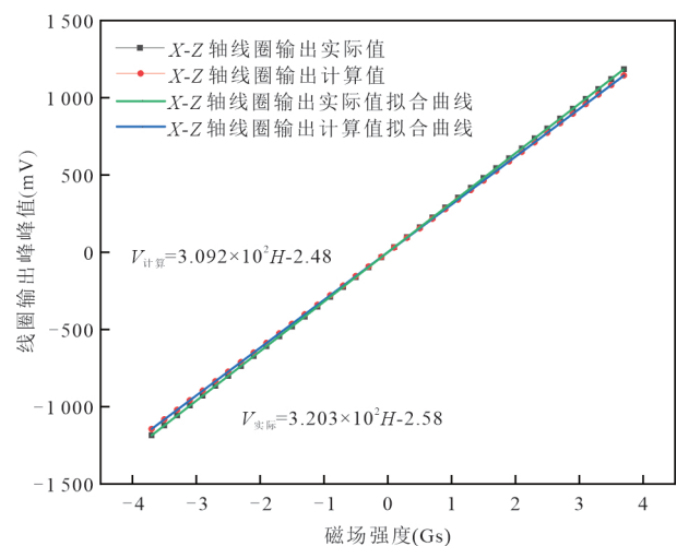
图8 X-Z轴探头线圈输出响应测量值与计算值对比曲线 Fig.8 Comparison curve of measured versus calculated values for X-Z axis probe coil output response
