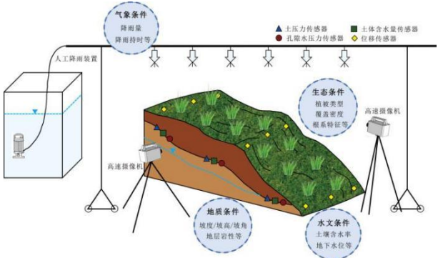
图 6 多因素耦合作用下滑坡物理模型试验概念图 Fig.6 Conceptual diagram of landslide physical model test under multi-factor coupling effect
