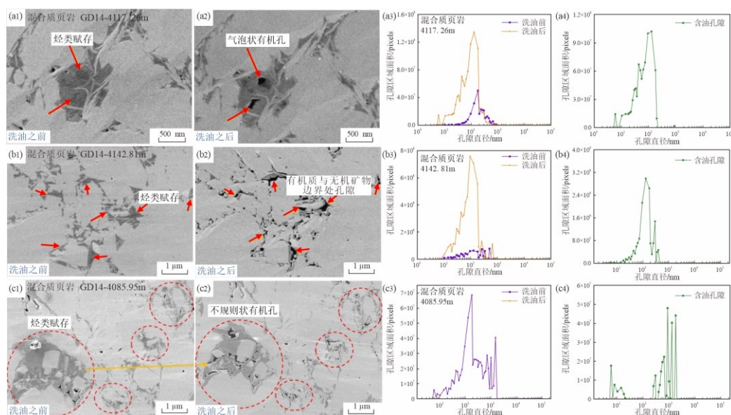
(a1, b1, c1) 洗油前页岩储层表面微观形貌; (a2, b2, c2) 洗油后页岩储层显露出次生有机孔 (烃类赋存空间); (a3, b3, c3) 洗油前后孔径分布曲线对比; (a4, b4, c4) 含油孔隙孔径分布曲线
