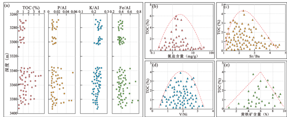
图 7 下干柴沟组上段烃源岩总有机碳含量与地球化学指标相关性分析图，修改自张斌等，2018；Liu et al. , 2016。（a）总有机碳与生产力指标；（b-c）总有机碳与盐度指标；（d-e）总有机碳与氧化还原指标 Fig.7 Correlation analysis diagram of TOC content and geochemical indicators in the upper member of Lower Ganchaigou Formation source rock, adapted from Zhang et al., (2018) and Liu et al., (2016). (a) TOC vs productivity indicators; (b-c) TOC vs salinity indicators; (d-e) TOC vs redox conditions
