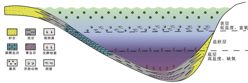
图3 咸化湖泊水体盐度分层、生物分层与沉积分异模式图，修改自 Guo et al., 2020, Liang et al., 2024 Fig.3 The schematic diagram of salinity stratification of water column, biological stratification, and sedimentary differentiation in saline lake, adapted from Guo et al., 2020 and Liang et al., 2024
