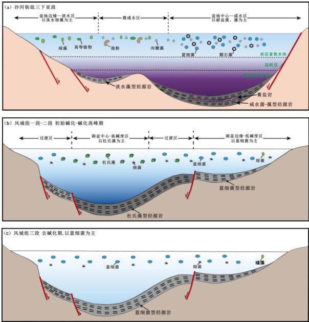
图 4 中国典型深时咸（碱）湖生物-环境协同变化模式图。（a）渤海湾盆地东濮凹陷沙河街组三下亚段沉积时期，修改自李红磊等，2020；（b-c）准噶尔盆地玛湖凹陷风城组沉积时期，修改自夏刘文等，2022 Fig.4 Synergistic change patterns diagram of biology and environment in typical deep-time saline (alkaline) lakes in China. (a) Sedimentary period of the lower third subsection of the Shahejie Formation in the Dongpu Sag of the Bohai Bay Basin, modified from Li et al.,2020; (b-c) Sedimentary period of the Fengcheng Formation in the Mahu Sag of the Junggar Basin, modified from Xia et al.,2022
