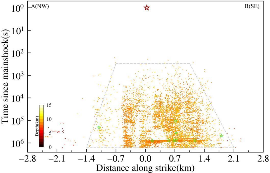
图 8 余震序列时空扩展分布 Fig.8 The occurrence times of aftershocks since the MuLi earthquake versus the along-strike distances
