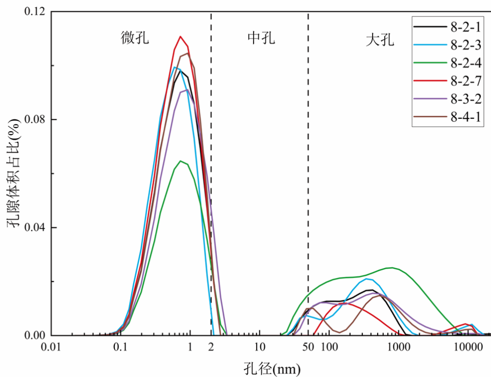
图 5 孔隙体积占比随孔径变化图 Fig. 5 Change in pore volume with pore size
